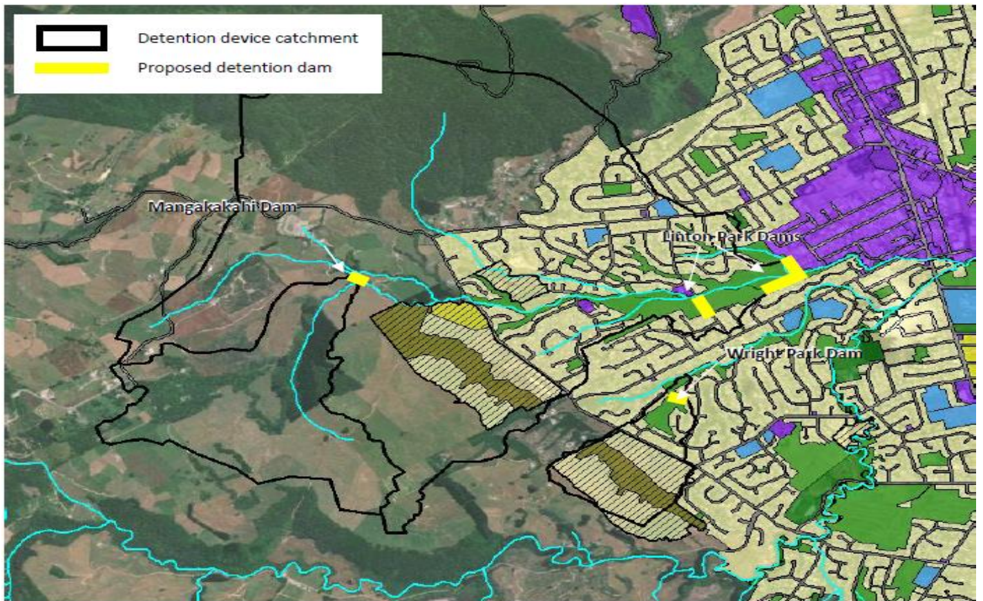
Figure 1. Location of the 4 proposed detention dams (Pukehangi PC2, West 04a, 04b & West 06)
