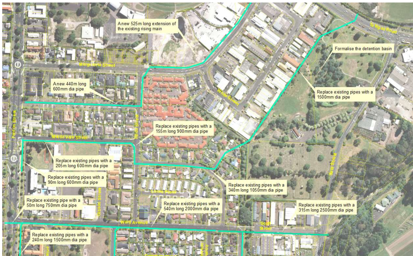
Figure 7a. Proposed upgrade works in sub-catchment 7 (Central 05 & 06)
