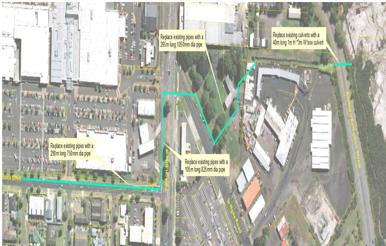
Figure 6c. Proposed upgrade works in sub-catchment 8 & 9 cont. (East section of Central 04)
