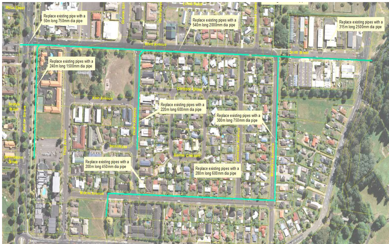
Figure 7b Proposed upgrade works in sub-catchment 7 (Central 05 & 06)
